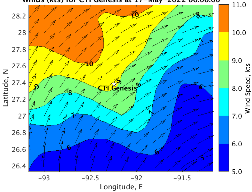
Winds (kts) for CTI Genesis at 17-May-2022 06:00:00
